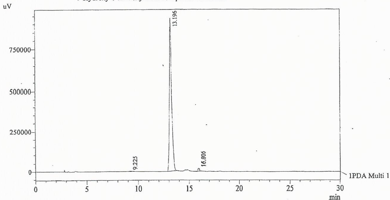
Chromatogram 4'-Hydroxy-6-methoxyflavone D:\promonence\Data
